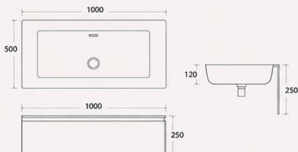
WASHBASIN (mm)
